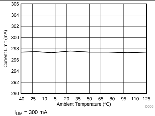
Figure 8. Current Limit vs Ambient Temperature
