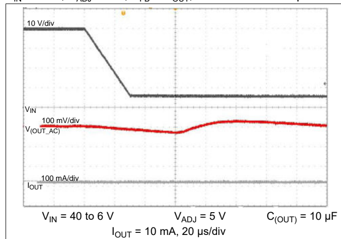
Figure 19. 40- to 6-V Line Transient
