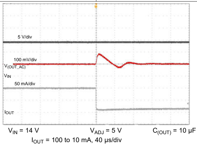
Figure 21. 100- to 10-mA Load Transient
