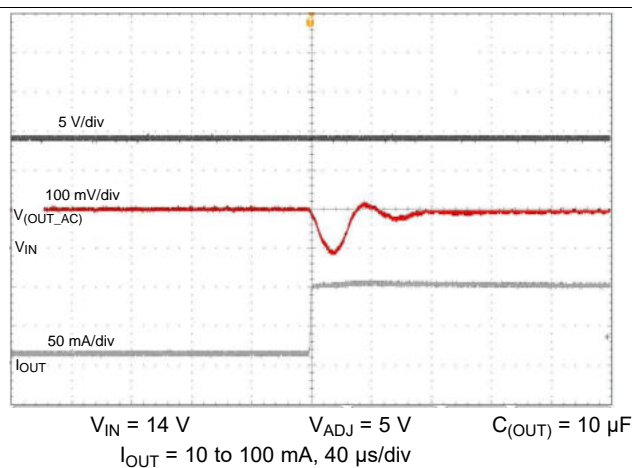
Figure 20. 10- to 100-mA Load Transient
