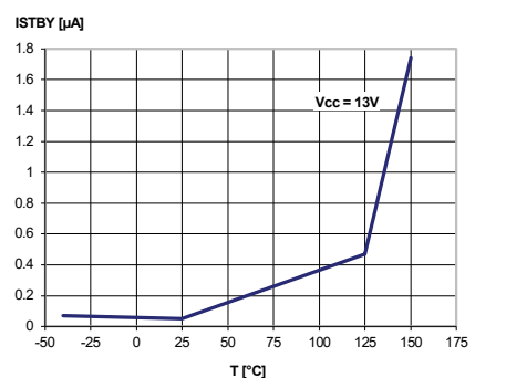
Figure 16: Standby current
