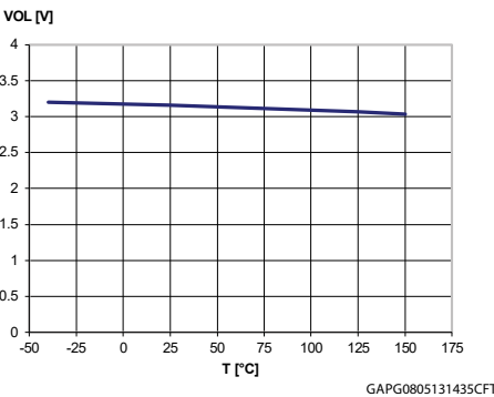
Figure 32: OFF-state open-load voltage detection threshold
