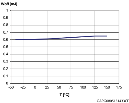
Figure 30: Woff vs. Tcase
