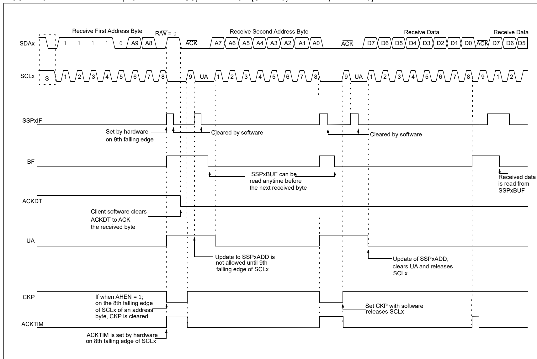
FIGURE 15-21: I 2 C CLIENT, 10-BIT ADDRESS, RECEPTION (SEN = 0, AHEN = 1, DHEN = 0)
